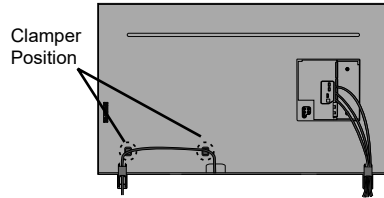
Type 1 (Outside pedestal)
